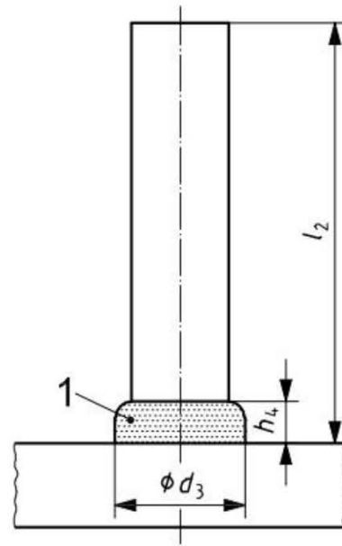
After welding
